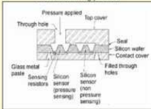
Figure 4: Cross section of 'g-insensitive' pressure sensor, showing top cover, silicon wafer and bottom mounting pedestal
