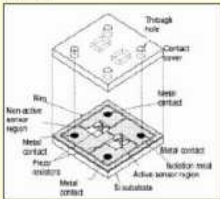
Figure 5: Silicon diaphragm showing piezoresistor sensor disposition, and contact cover by means of which sensor is mounted
