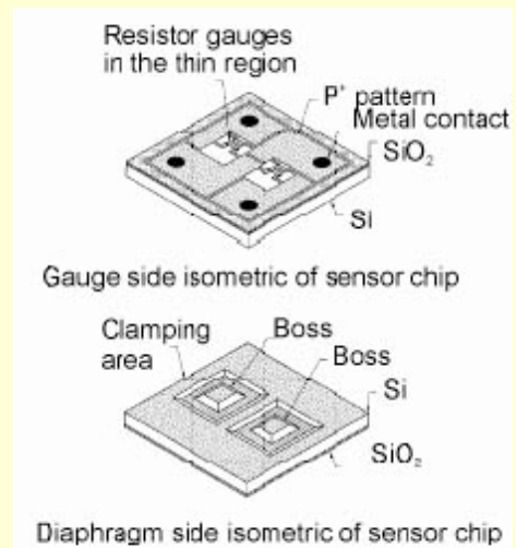
Figure 7: Isometric views of silicon chip showing piezoresistor side and etched diaphragm side
