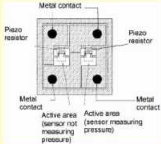
Figure 6: Plan view of silicon chip showing the two adjacent active areas, one only of which is exposed to pressure.
